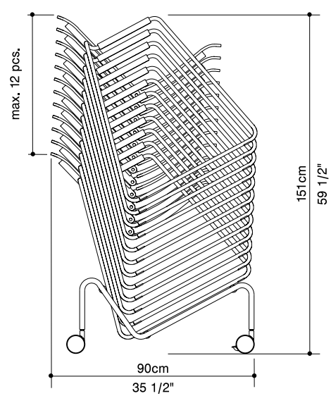
ST.HC with 12 SEATTABLES stacked as chairs
